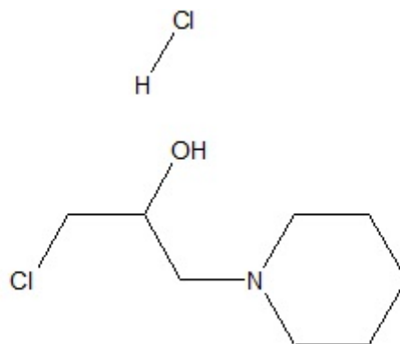
N-(3-Chloro-2-hydroxypropyl)-piperidine hydrochloride
